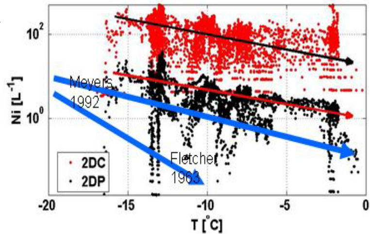
ISDAC-April 24 FLT#28 2008
