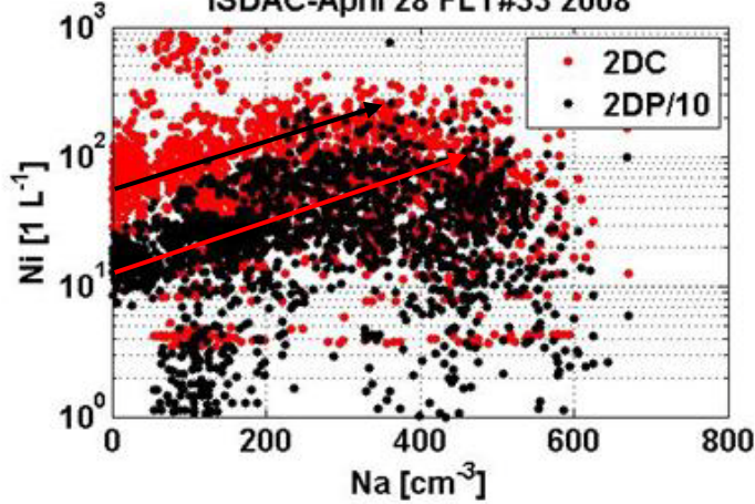
ISDAC-April 28 FLT#33 2008
