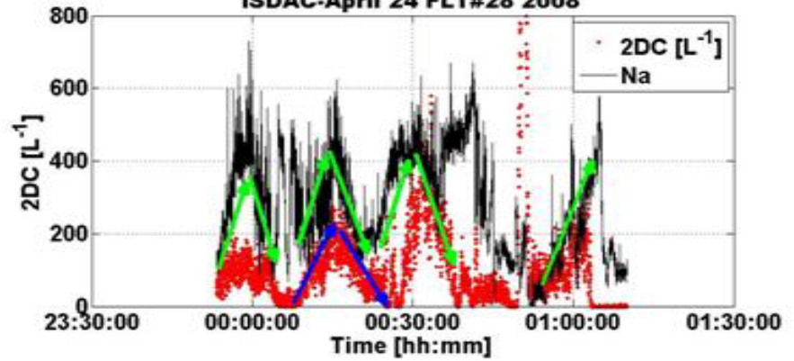
ISDAC-April 24 FLT#28 2008
