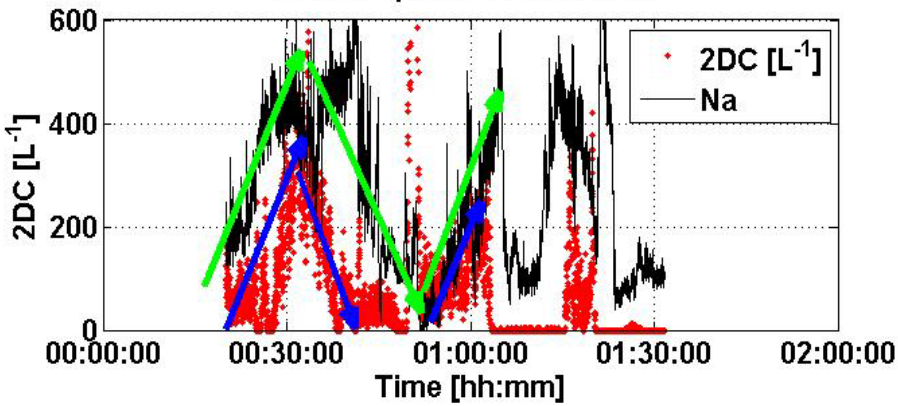
ISDAC-April 28 FLT#33 2008
