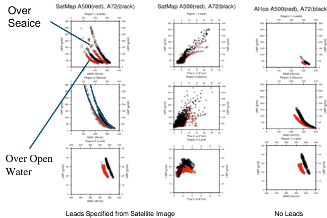
Sensitivity of downward surface shortwave radiation and precipitation to small mode aerosol concentration at 21Z April 8 2008
