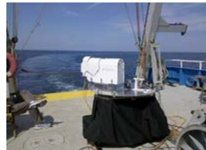
The AMF2 stable platform at sea aboard the RV Connecticut during a three-day cruise out of Woods Hole. The MWR, MFRSR, and a tilt sensor are in place and operating on the platform, which includes a turntable to compensate for ship yaw.
