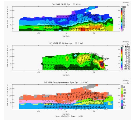
Cross-sections of reflectivity and airflow (top panel), vertical motion and airflow (middle panel), and hydrometeor type and airflow (bottom panel) for the 20 May MCS observed in MC3E.
