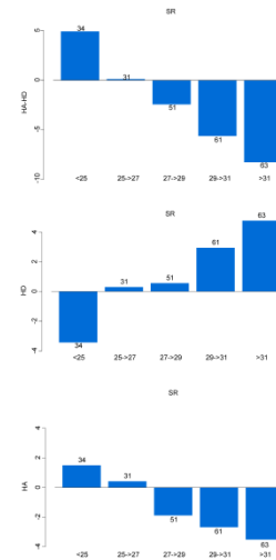
Figure 1. Mean daily values of HA - HD (top), HD (middle), and HA (bottom) when the mean daily solar radiation ( SR ) was in one of five categories shown. The abbreviations for these variables are defined in the text. The daily values are areal averages over our study region from all eight study months. The numbers on the top of the bars indicate the number of days that were included in that SR category. SR is in MJ\ m^{-2}\ day^{-1} with all other variables having units of mm\ day^{-1} .
