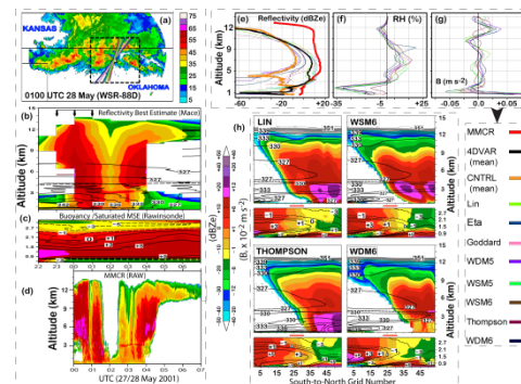
Figure 1. Observed (left) and simulated (right) reflectivity and thermodynamic structure for the SGP CF for 2300 UTC 27 May–0100 UTC 28 May 2001.
