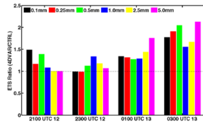
Figure 1. The ratio of equitable threat scores (ETS), defined as R = ERS4DVAR/ETSCTRL for 1-hour accumulated precipitation between CTRL (without assimilation of wind profiles) and 4DVAR (with assimilation of wind profiles) experiments with threshold of 0.1, 0.25, 1.0, 2.5, and 5.0 mm at 2100 UTC 12 June 2002, 2300 UTC 12 June 2002, 0100 UTC 13 June 2002, and 0300 UTC 13 June 2002. When ETS ratio is greater than 1, the QPF skill is improved by 4DVAR.
