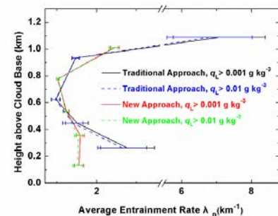
Figure 1. Comparison of the vertical profile of entrainment rate ( \lambda_p ) obtained using the new approach and the result from a traditional approach with different liquid water mixing ratio thresholds. The uncertainties are also shown.
