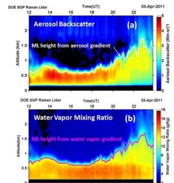
(a) SGP Raman lidar aerosol backscatter (355 nm) measurements on April 3, 2011. A preliminary indication of the mixing layer (ML) height as determined from the gradient in aerosol backscatter is shown by the white line. (b) Same except for SGP Raman lidar measurements of water vapor mixing ratio.
