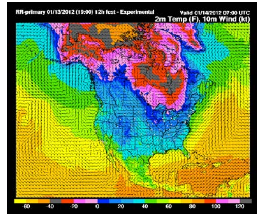
Experimental RAP 12-h forecast: 2-m temperature, and 10-m wind.
