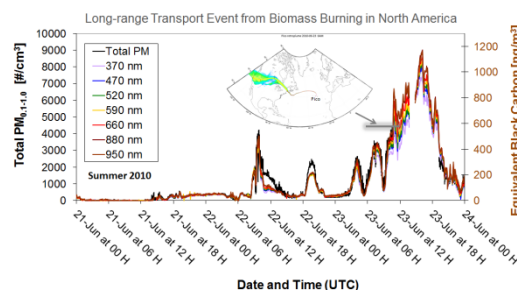
Long-range transport event from biomass burning in North America to the Pico Mountain Observatory in the Azores, Portugal.
