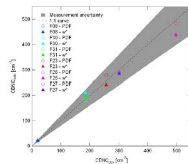
Figure 1: Comparison of cloud droplet number concentrations (CDNC), calculated using an adiabatic parcel model with two different representations of the updraft velocity, with CDNC values observed in-cloud. Six cases during ISDAC are considered: three from flights in clean aerosol conditions (F08, F30, F31) and three from flights in polluted aerosol conditions associated with biomass burning plumes (F23, F26, F27).
