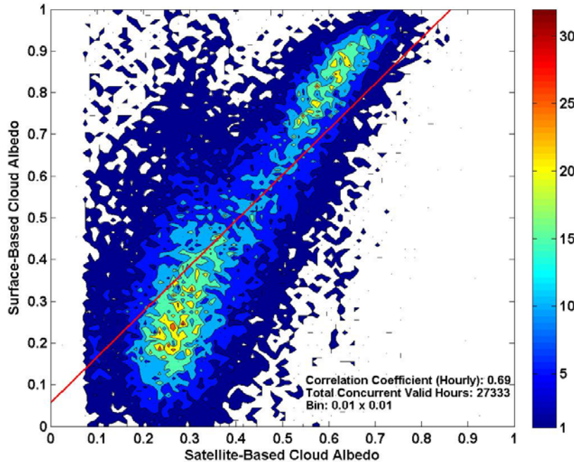
Cloud Albedo
