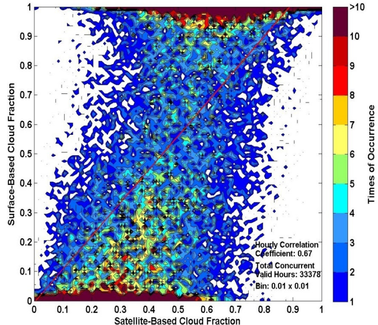
Cloud Fraction
