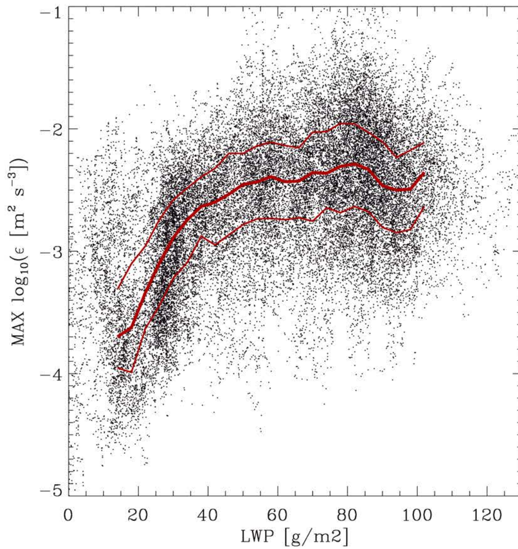
Max \epsilon vs. LWP
