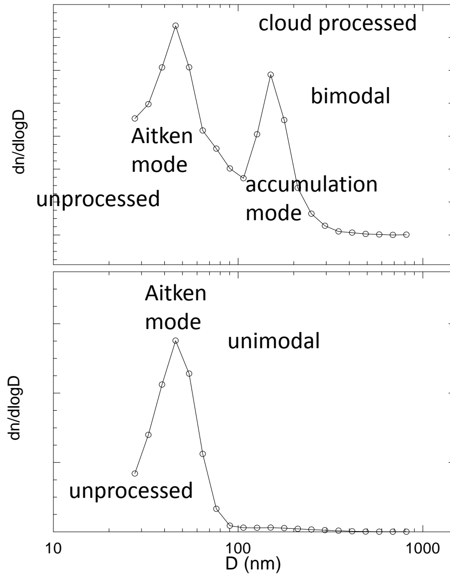
Figure 1. Examples of SMPS spectra at SGP, May 2003
