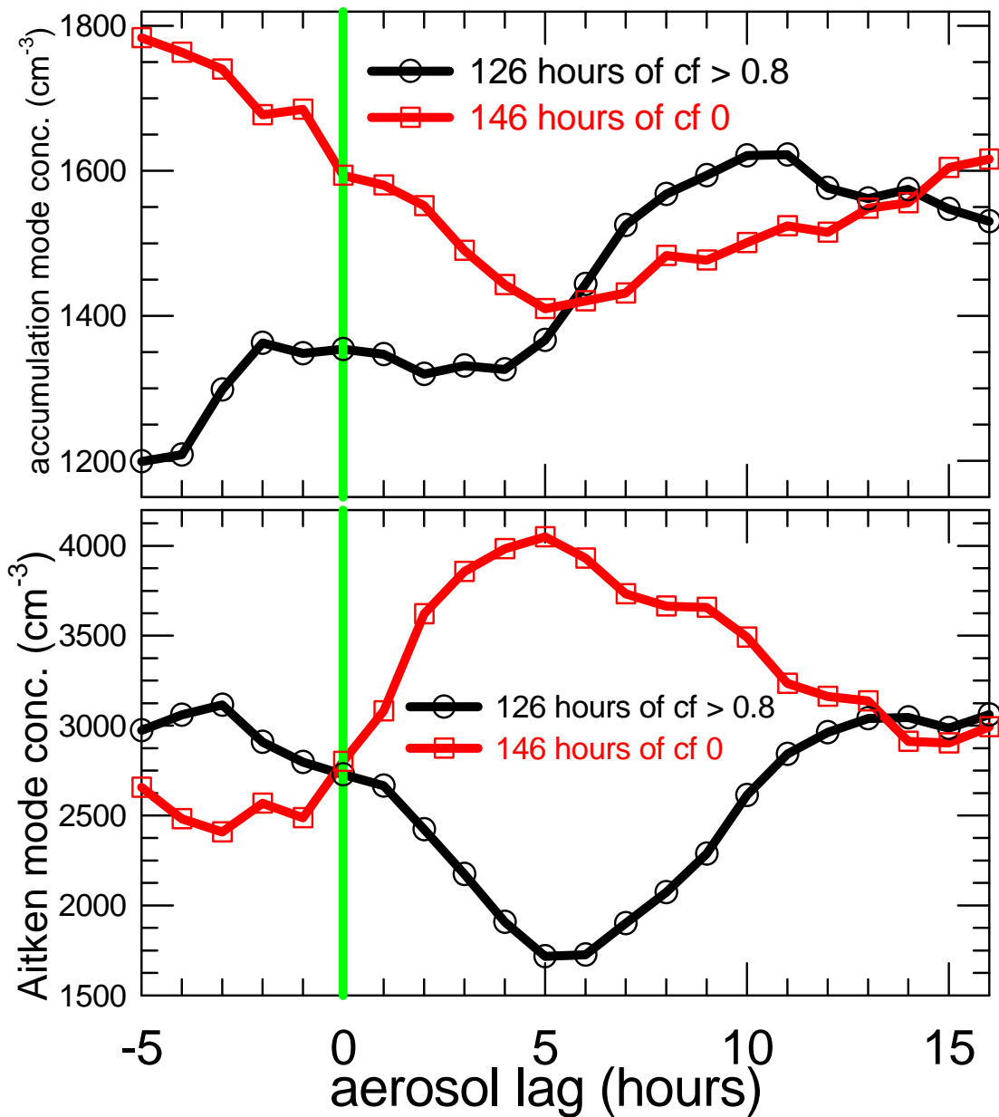
Figure 4. Mean surface particle concentrations within the two aerosol modes as a function of time after the specific ceilometer cloud fractions (CF) have been remotely observed at time zero (green line).
