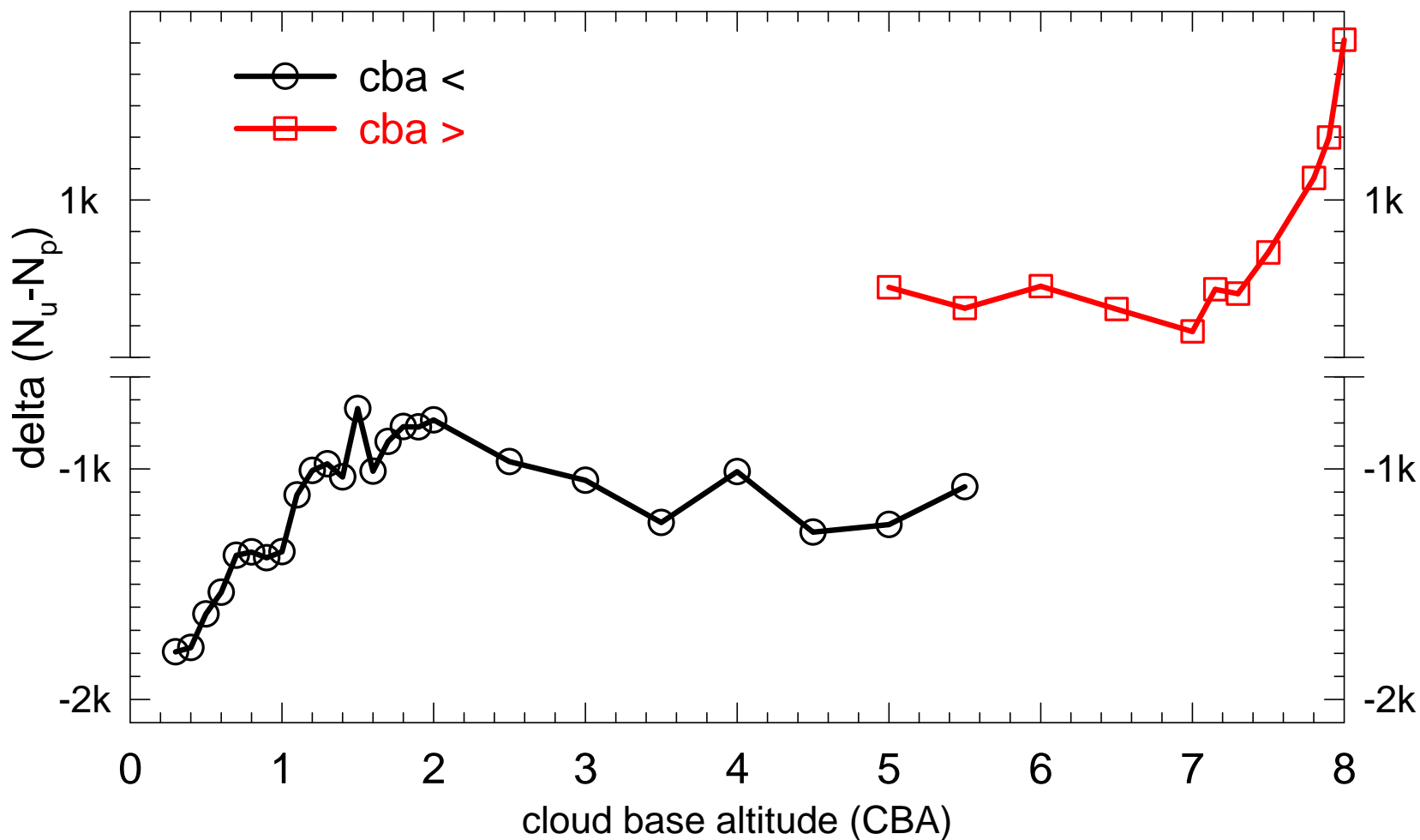
Figure 5. Differences between mean normalized modality [(N_u - N_p)/(N_u + N_p)] at 0 hour from mean normalized at lag hour of minimal normalized (black) for all cases with cloud base altitude (CBA) less than the abscissa designation. This indicates progressively greater bimodality for progressively lower CBA. Red are the differences between mean normalized at 0 hours from mean normalized at lag hour of maximal normalized for all CBA greater than abscissa; this indicates progressively greater unimodality for progressively higher CBA. Lower CBA is similar to higher CF in terms of causing aerosol bimodality. The modality differences so described come from figures such as Fig. 3 for various CBA taking the difference between concentrations at zero hour and at minimum (black) and maximum (red).
