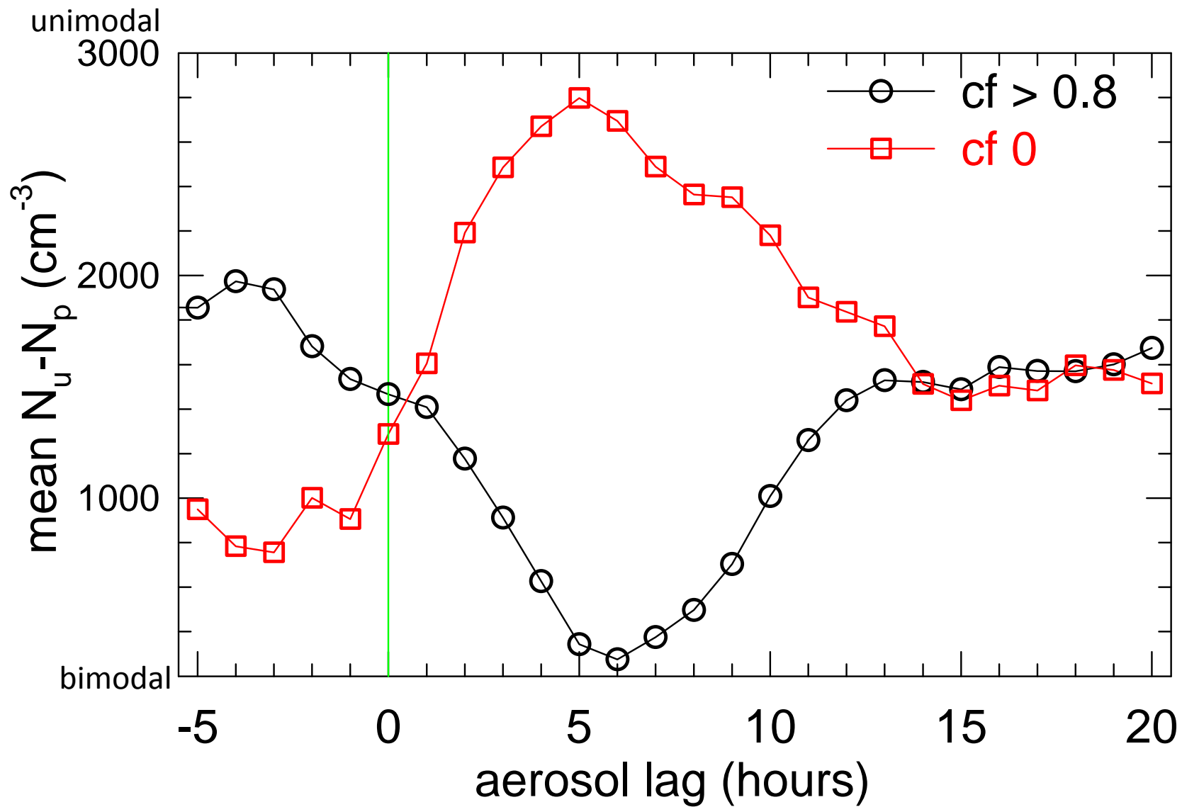
Figure 3. Mean aerosol bimodality ( N_u - N_p ) lagged response of 234 hours of surface aerosol to extreme cloud fractions (CF). 88 hours of CF > 0.8, 146 hours of zero CF. Lower N_u - N_p is bimodal; higher N_u - N_p is unimodal. Bimodal response to high CF, unimodal response to low CF.
