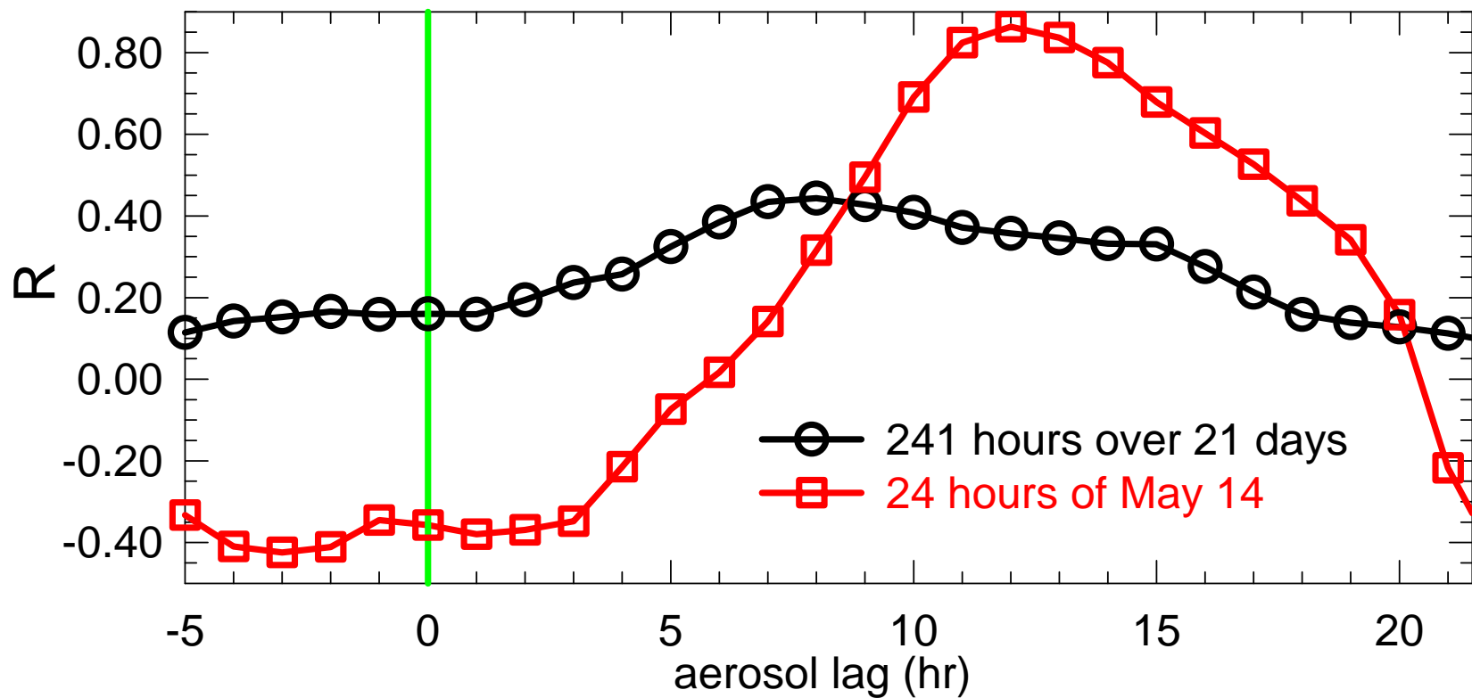
Figure 2. Correlation coefficients ( R ) between hour averages of surface SMPS aerosol modality (bimodal versus unimodal) with PGN remote measurements of cloud fraction (CF) plotted against time lag of aerosol data from the cloud data at zero hour (green line). Aerosol modality is in terms of the concentration differences between Aitken particles (smaller than Hoppel minima; not cloud-processed; N_u ) and accumulation mode particles (larger than Hoppel minima; cloud-processed; N_p ). R s are higher for time lags necessary for the surface aerosol to respond to specific CF mainly by advecting to the surface.
