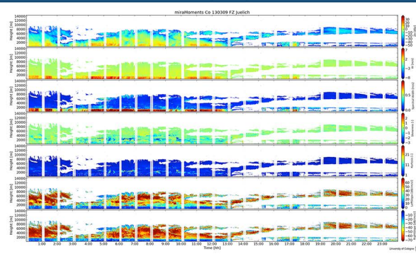
An updated data processing of the cloud radar MIRA@JOYCE now allows to retrieve higher spectral moments (kurtosis, panel 4 & skewness, panel 5) of the Doppler spectrum along with "usual" values of reflectivity (panel 1), Doppler velocity (panel 2) and Doppler velocity spectral width (panel 3). In precipitation, the left (panel 6) and right (panel 7) slope of the most significant peak in the Doppler spectrum shows potential to infer extended information on the particle size spectrum microphysics. Additionally, the full velocity co- and cross-spectra are stored using an optimized compression.
