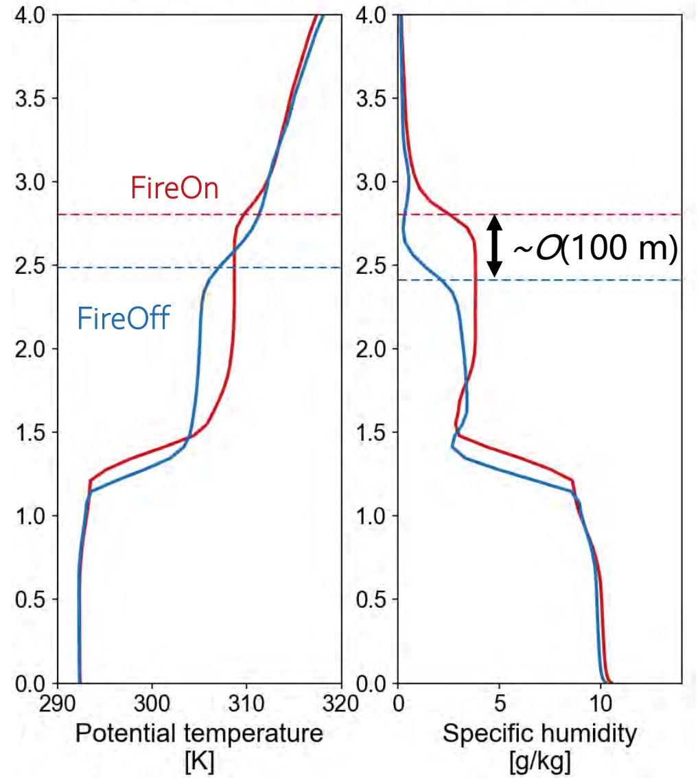
WRF FireOn and FireOff 2017-08-16T20:00 to 2017-08-16T21:00
